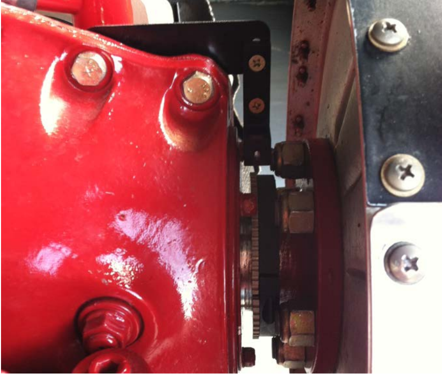
Figure 3: With Magnetic Sensor & Bracket Installed
